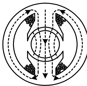
Simple motor geometry
